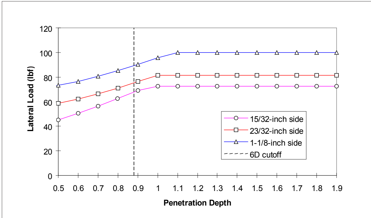
Figure 1. Lateral load of a single 10d nail as a function of nail penetration and side member thickness. Side member and main member have assumed SG = 0.42.
